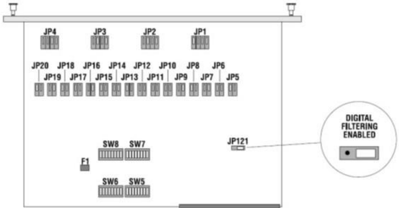
Figure 14 Configuration Jumper Locations
