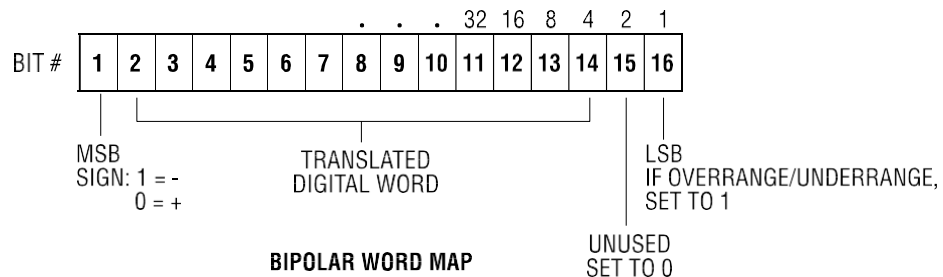
Figure 4 Word Input to the PLC from the Module (Bipolar)
