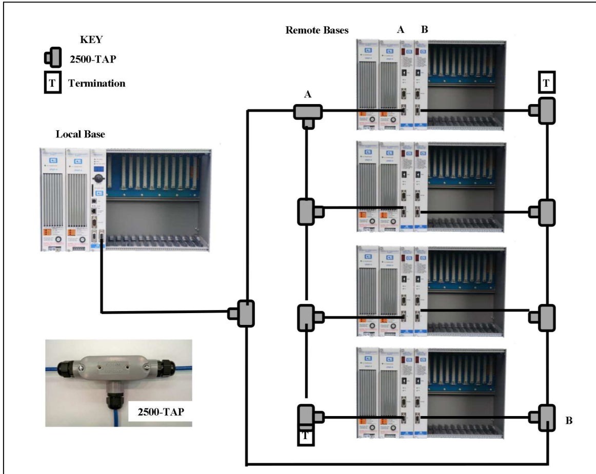
Figure 1: Typical Dual Media Redundancy Layout
