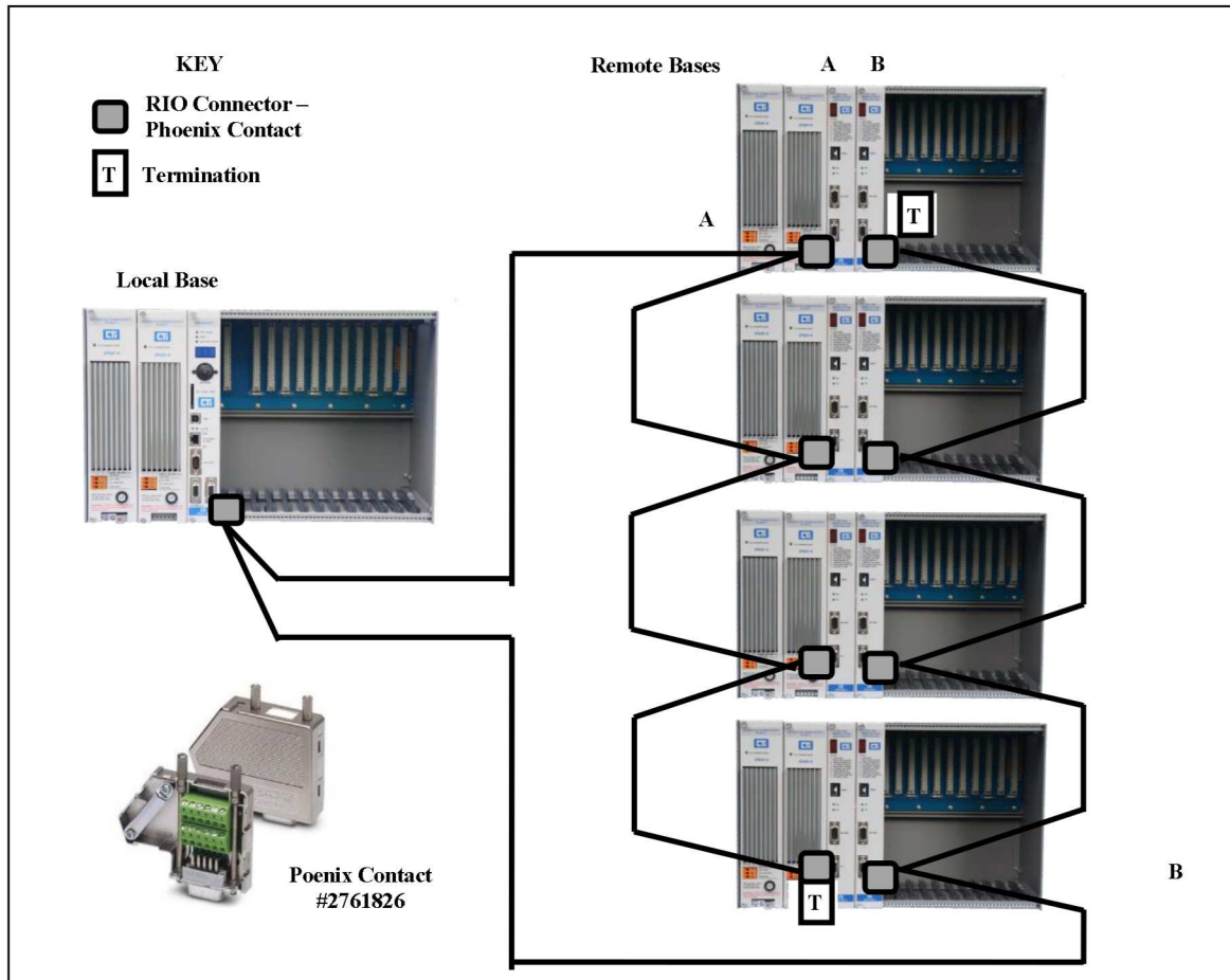
Figure 2: Recommended Dual Media Redundancy Layout
