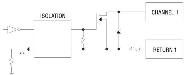
2591-A Typical Internal Circuit
