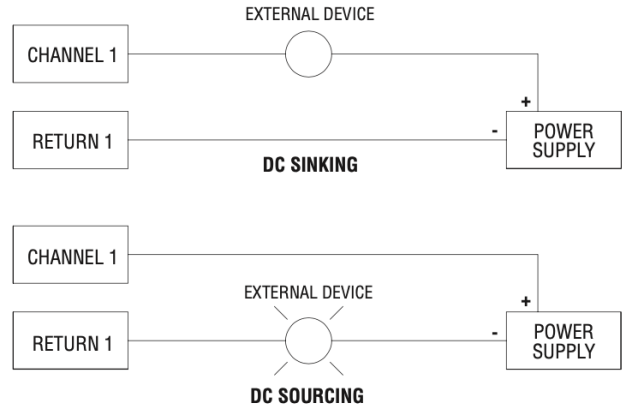
2591-A Typical External Wiring Application
