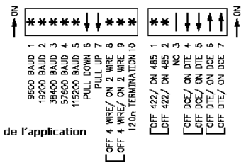
Configuration des DIP Switch ICM5
