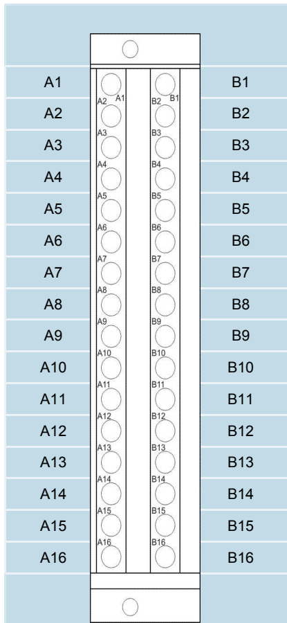
2500C-32F Wiring Connector
