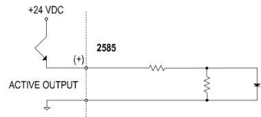
TYPICAL CONNECTION FOR HIGHER LEVEL VOLTAGE (24 VDC)
