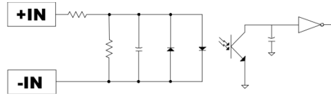
Typical Circuit
