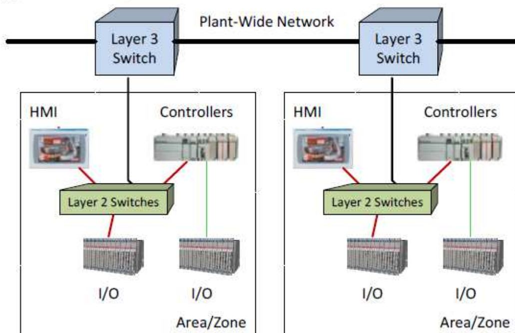
Figure 1: Subdivided plant network.
